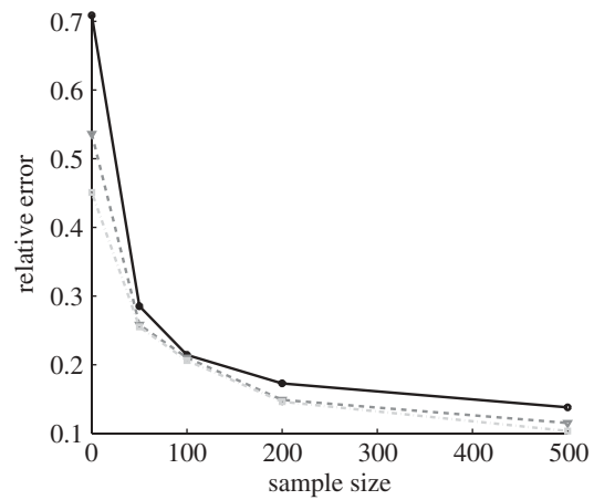
Figure 5. Simulation study of estimation of the next-generation matrix \beta using our maximum likelihood method. Generating
