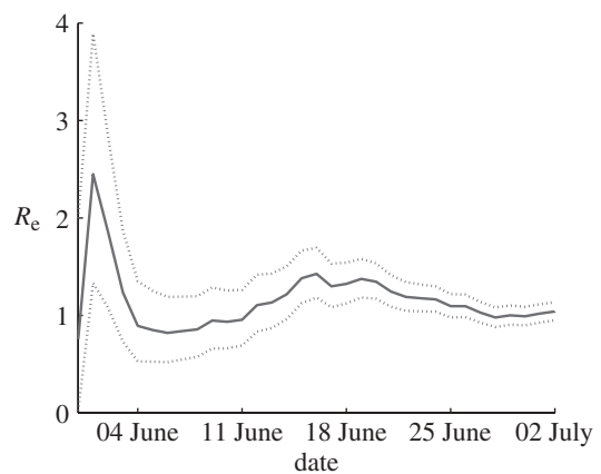
Figure 4. Changes in R_e estimates as the epidemic progresses. For each day, starting from 30 May, R_e is estimated based on the time series initiating on 20 May up to that day. The solid line depicts the estimated R_e values and the dashed lines the 95% Bayesian lower and upper credibility intervals.
