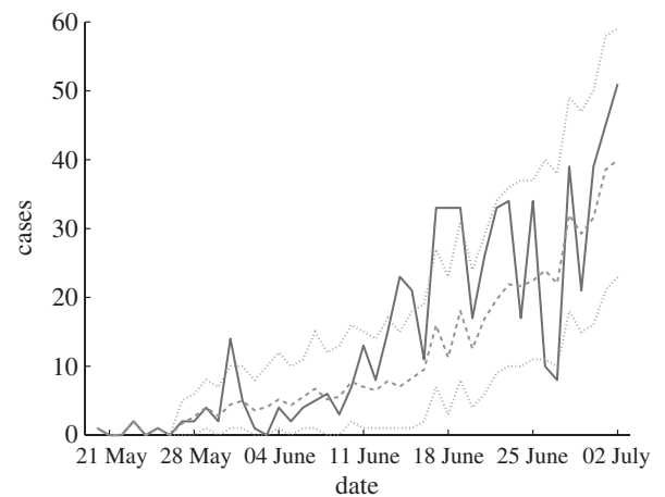
Figure 3. Confirmed 2009 H1N1 cases (solid line), with the simulation curve obtained by averaging 1000 simulations of the stochastic model (2.2) using the estimated R_e (dashed line), together with 95% bands (dotted lines).
