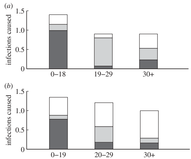
Figure 6. (a) Representation of the estimated next-generation matrix \beta : each bar represents the average number of infections caused by a single infected individual of the corresponding age group in each of the age groups. (b) Representation of the next-generation matrix based only on social contacts as derived from the POLYMOD study [37]. The ages are grouped slightly differently than in (a) since the social contact matrices in this study were given in 5-year age bands (filled dark grey region, 0–18; filled grey region, 19–29; white region, 30+).
