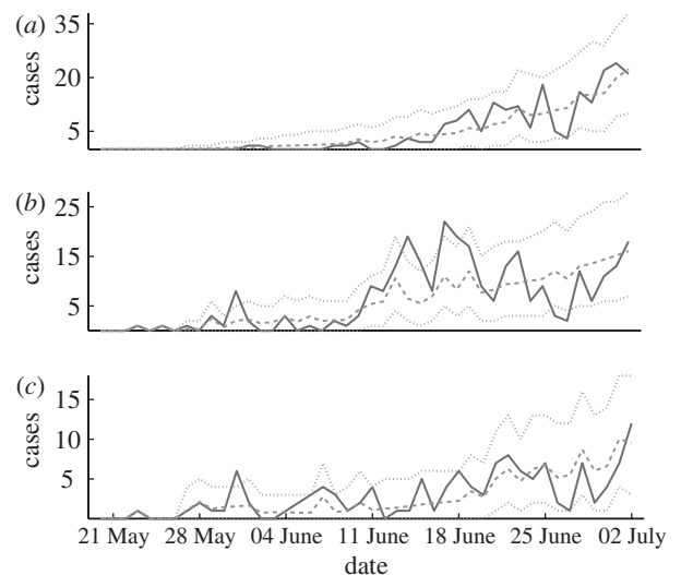
Figure 7. Confirmed 2009 H1N1 cases in each age group (solid line) and the simulation curve obtained by averaging 1000 simulations of the stochastic age group model (3.3) using the estimated matrix \hat{\beta} (dashed line), together with 95% bands (dotted lines). (a) 0–18 age group, (b) 19–29 age group and (c) 30+ age group.
